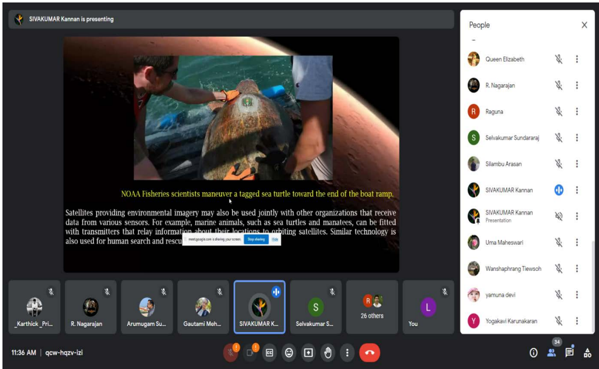
Webinar Session on Monitoring of the Sea Turtle by tagging technique
