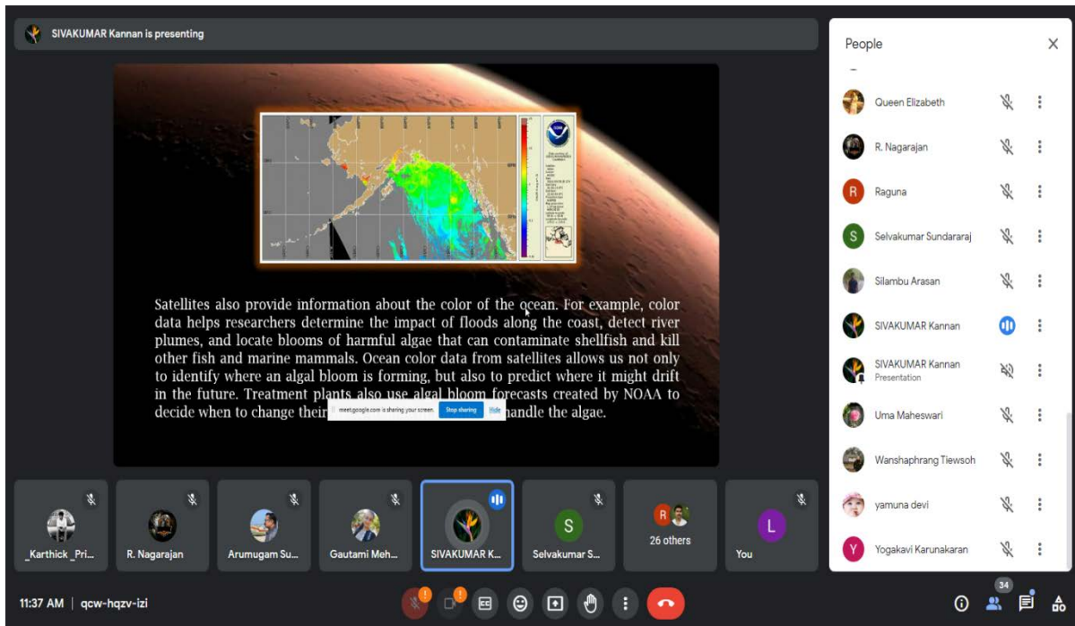
Webinar Session explaining about harmful algae blooms
