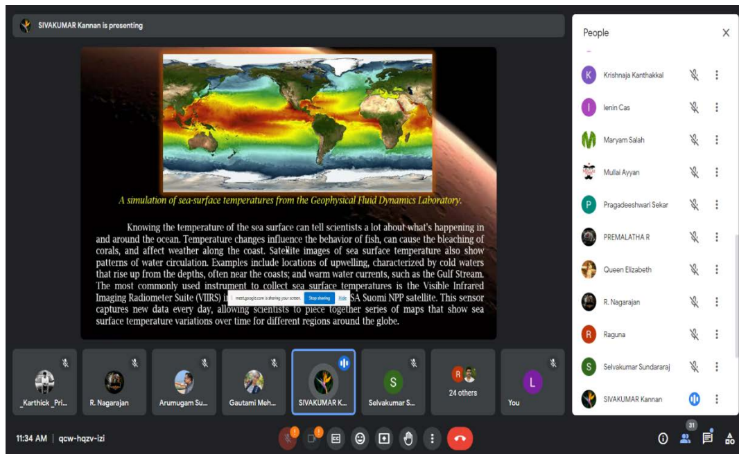
Dr. K. Sivakumar explaining about Sea Surface Temperature
